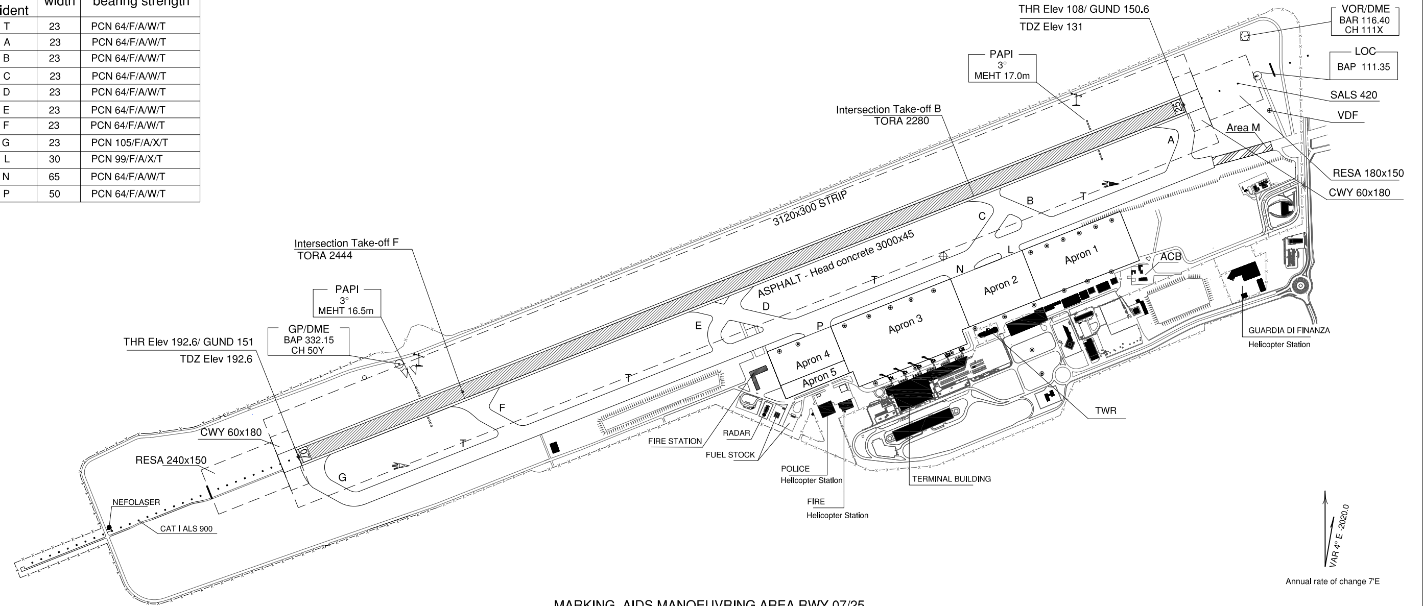
MARKING AIDS MANOEUVRING AREA RWY 07/25
