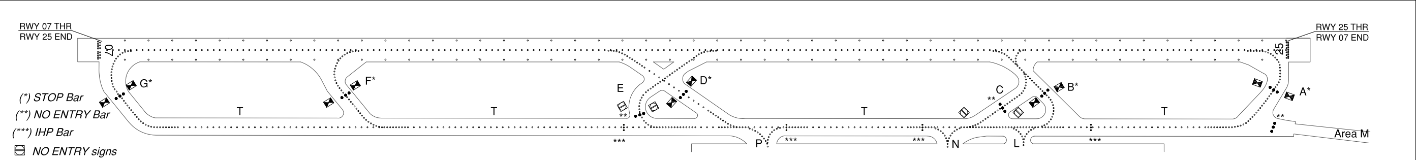
LIGHTING AIDS MANOEUVRING AREA RWY 07/25
